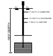
BORE WELL DETAILS
