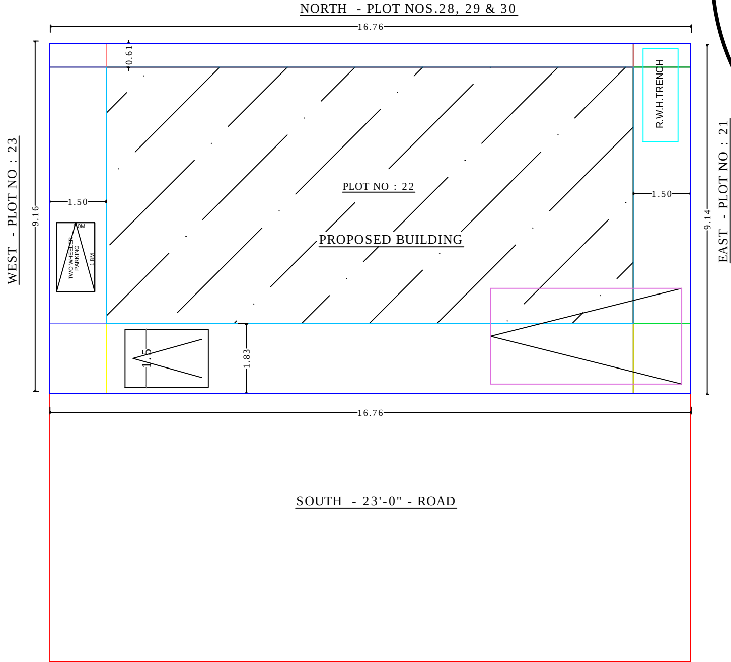
SITE PLAN
