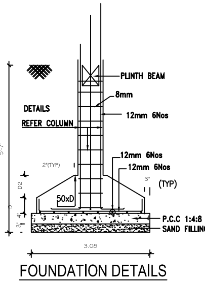
FOUNDATION DETAILS
