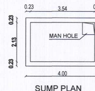
PLAN SUMP
