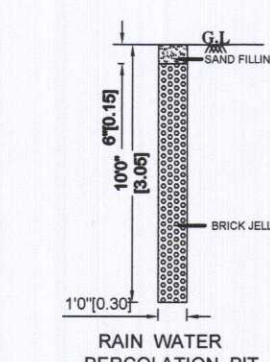
RAIN WATER PERCOLATION PIT
