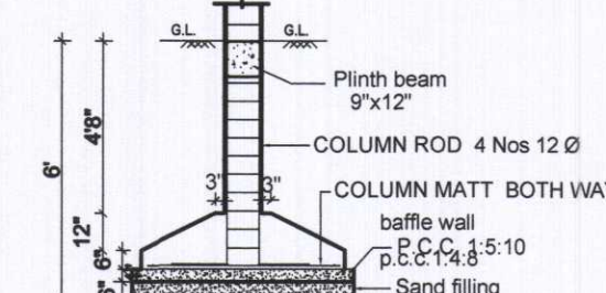
SECTION COLUMN
