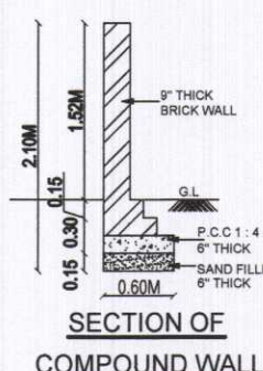
SECTION OF COMPOUND WALL
