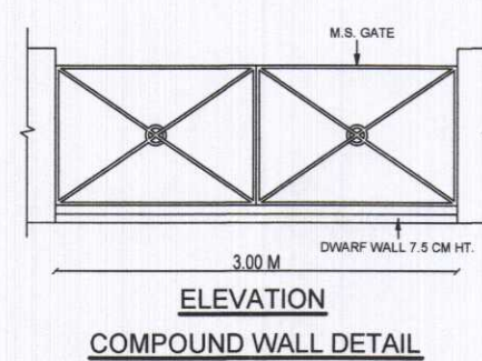
ELEVATION COMPOUND WALL DETAIL
