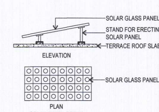
SOLAR PANEL DETAIL
