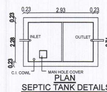
PLAN SEPTIC TANK DETAILS
