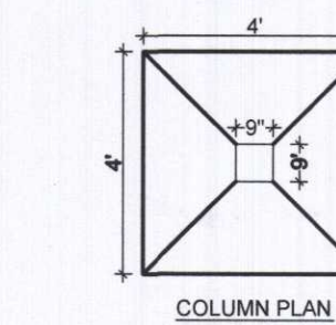
PLAN COLUMN
