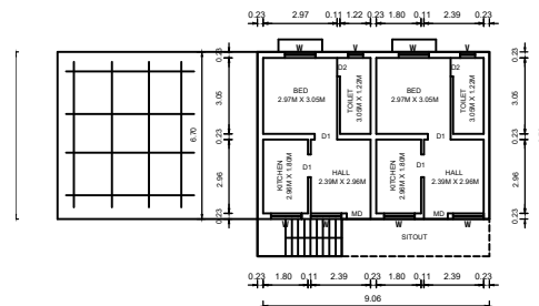
PRO. FIRST FLOOR PLAN
