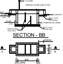
PLAN OF SEPTIC TANK
