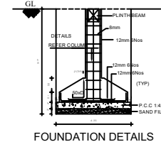
FOUNDATION DETAILS
