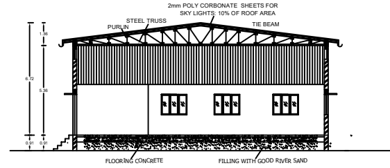
SECTION ON "MS"
