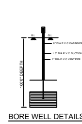
BORE WELL DETAILS
