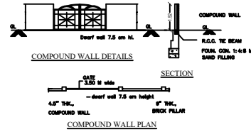
COMPOUND WALL PLAN
