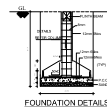
FOUNDATION DETAILS
