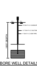
BORE WELL DETAILS
