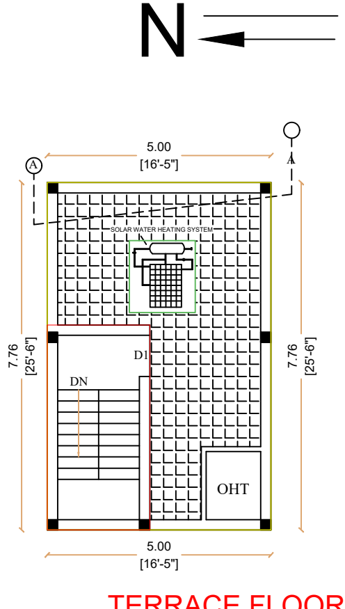
TERRACE FLOOR
