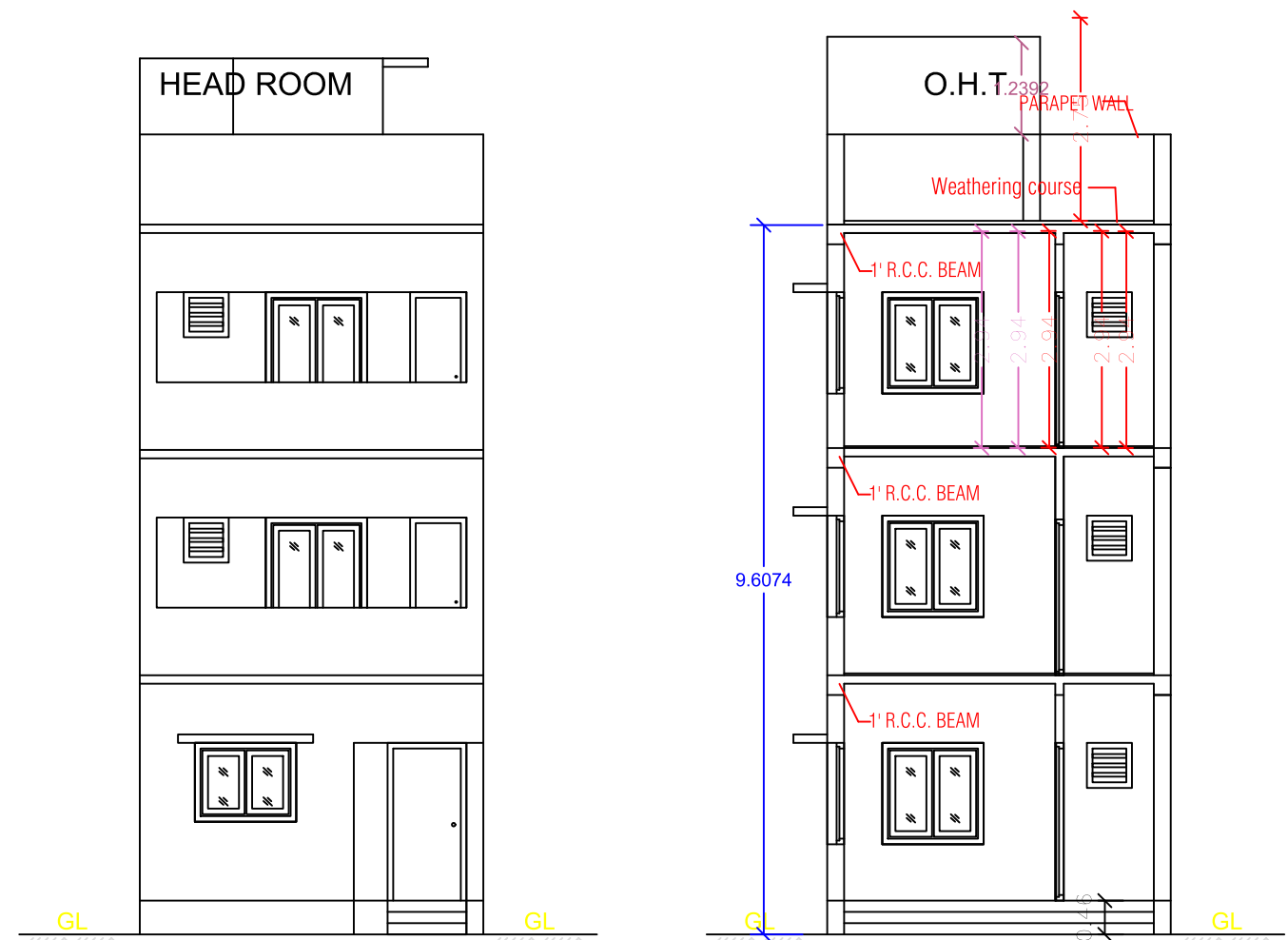
FRONT ELEVATION
