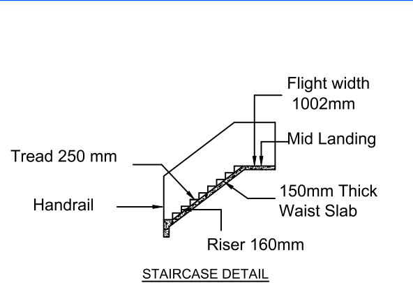
STAIRCASE DETAIL
