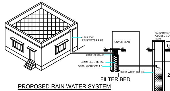
RAIN WATER SYSTEM
