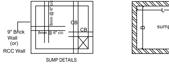
SUMP DETAILS
