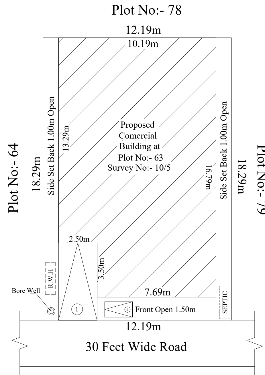
SITE PLAN
