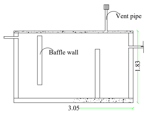
SEPTIC TANK DETAILS Size: 3.05 x 1.83 SCALE 1:100
