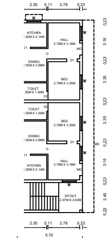
PRO. FIRST FLOOR PLAN
