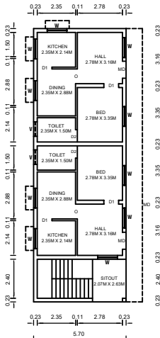
PRO. SECOND FLOOR PLAN
