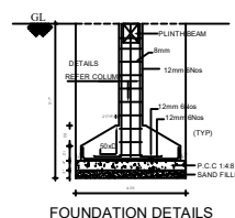
FOUNDATION DETAILS
