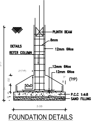
FOUNDATION DETAILS
