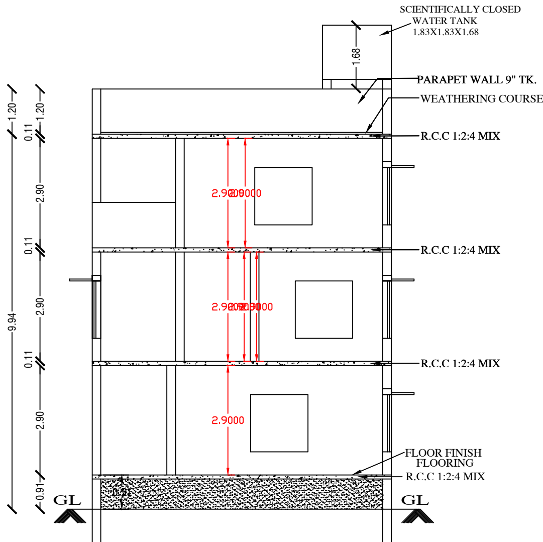
SECTION : "A-A"
