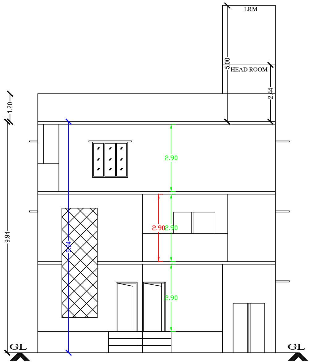
FRONT ELEVATION
