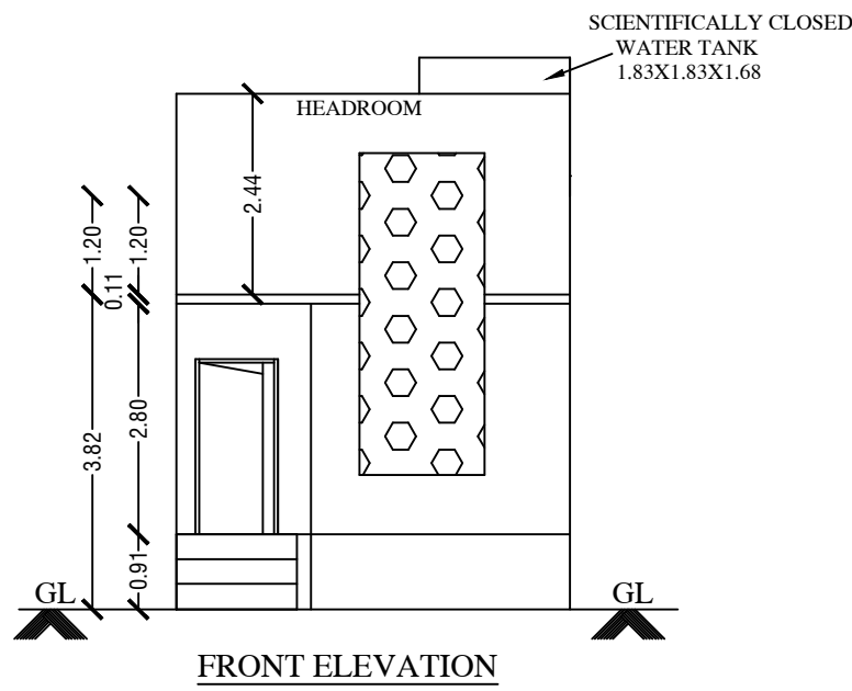
FRONT ELEVATION
