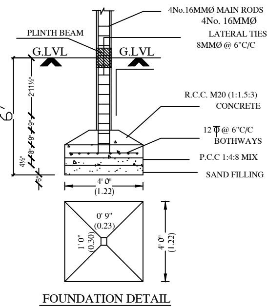
FOUNDATION DETAIL (SCALE: 1/30)
