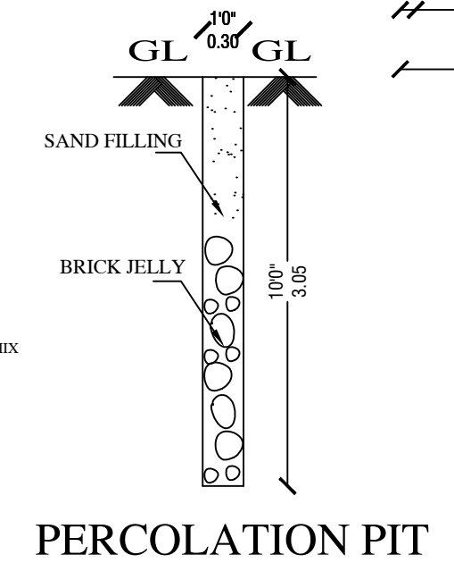
PERCOLATION PIT
