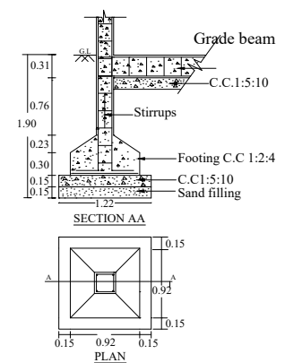
FOUNDATION DETAILS
