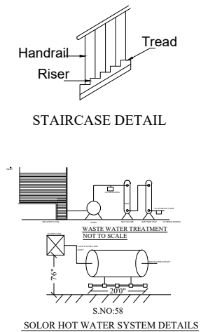
SOLAR HOT WATER SYSTEM DETAILS
