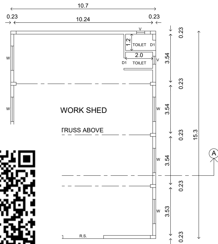
FLOOR PLAN 100
