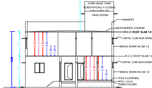
SECTION AB
