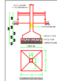
FOUNDATION DETAILS
