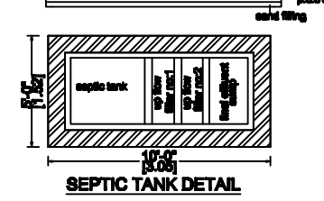
SEPTIC TANK
