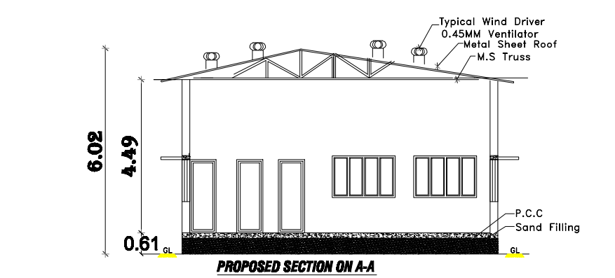
PROPOSED SECTION ON A-A
