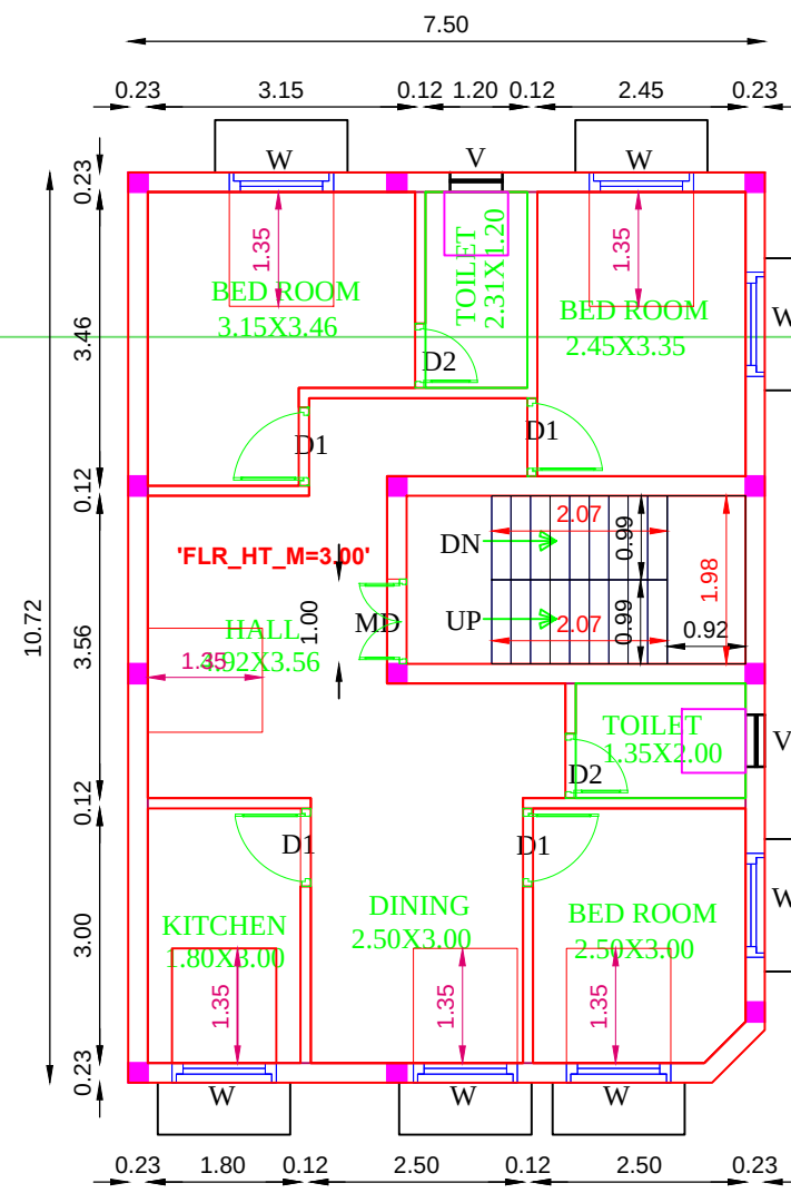
SECOND FLOOR PLAN [PROPOSED]
