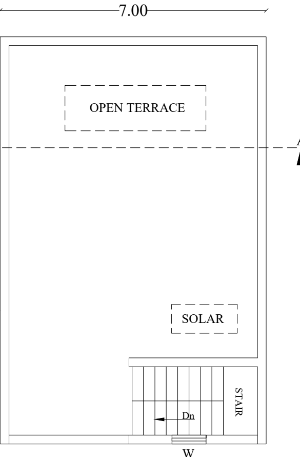
TERRACE FLOOR
