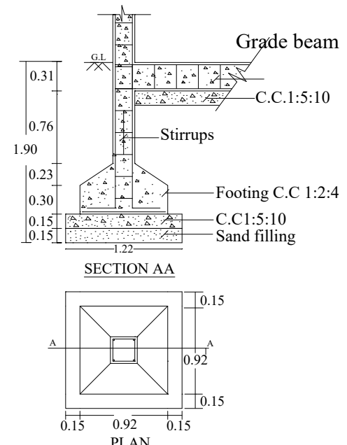
FOUNDATION DETAILS
