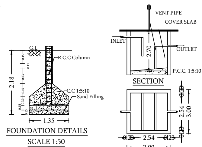
FOUNDATION DETAILS SCALE 1:50
