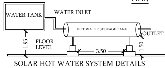
SOLAR HOT WATER SYSTEM DETAILS
