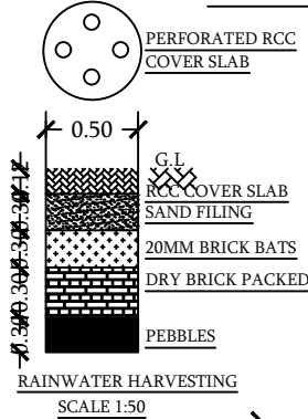
RAINWATER HARVESTING SCALE 1:50
