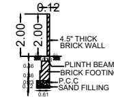
COMPOUND WALL
