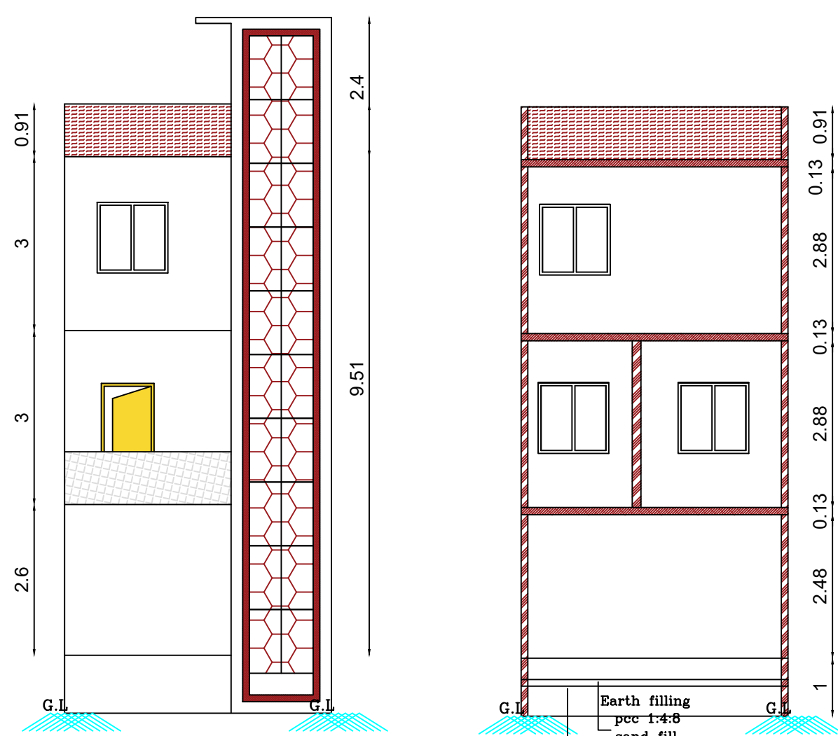
ELEVATION-AA
