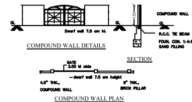
COMPOUND WALL PLAN
