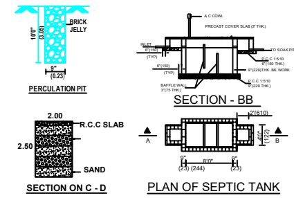
SECTION ON C - D
