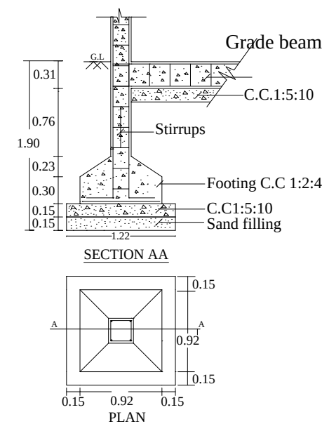
FOUNDATION DETAILS
