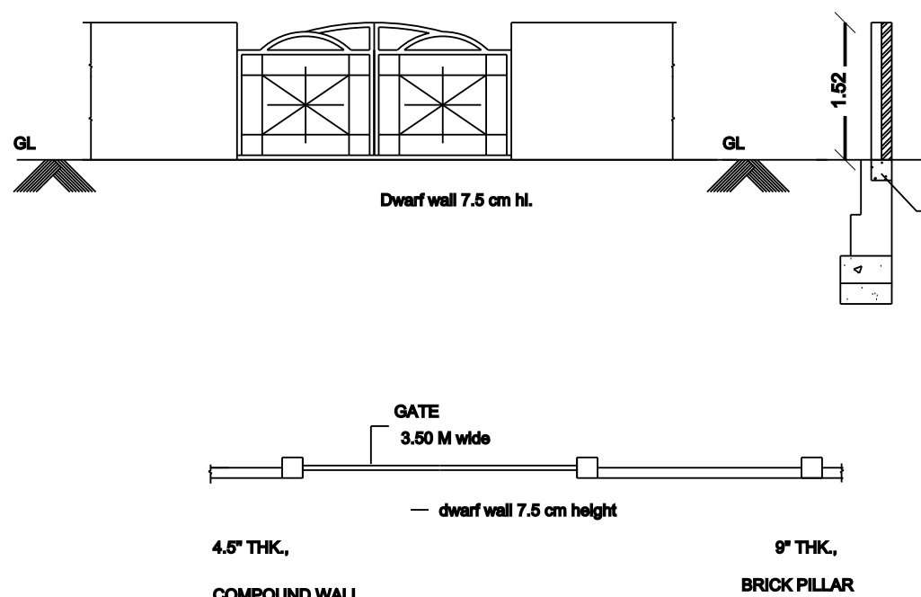
FOUNDATION DETAILS
