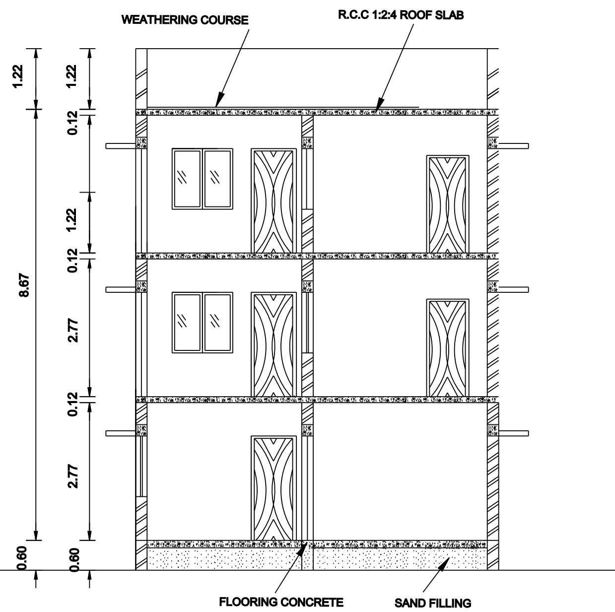
SECTION ON " MS "
