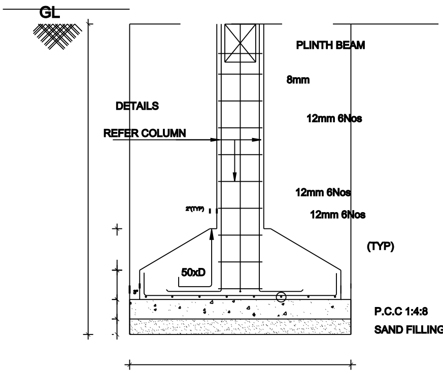
FOUNDATION DETAILS
