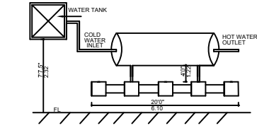
SOLAR HOT WATER SYSTEM DETAILS
