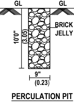
PERCULATION PIT
