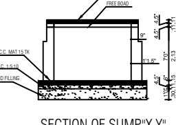
SECTION OF SUMP
