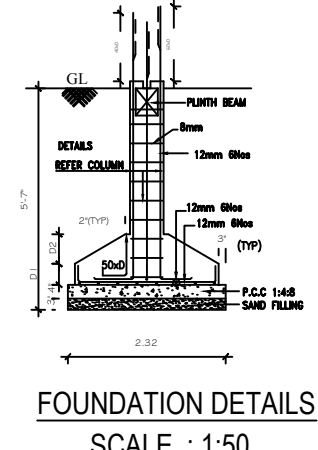
FOUNDATION DETAILS SCALE : 1:50.
