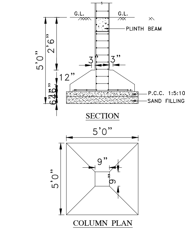
TYPICAL FOUNDATION DETAIL
