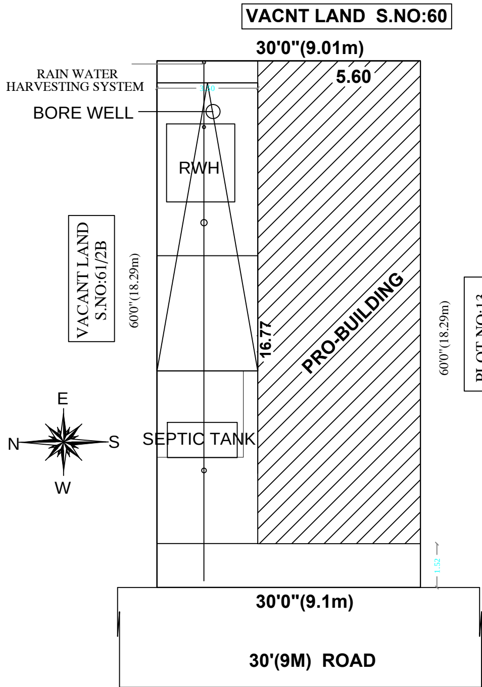
SITE PLAN
