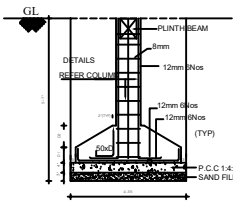
FOUNDATION DETAILS
