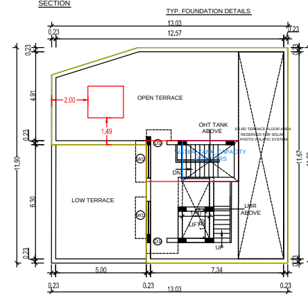
TERRACE FLOOR PLAN (PROPOSED)
