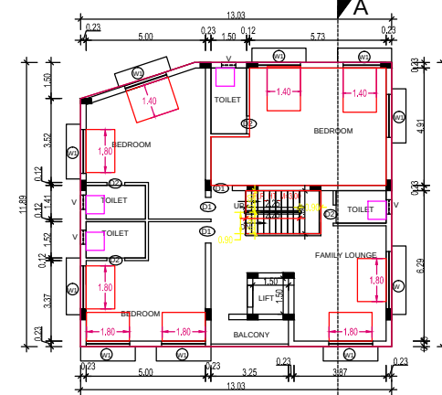
SECOND FLOOR PLAN (PROPOSED)
