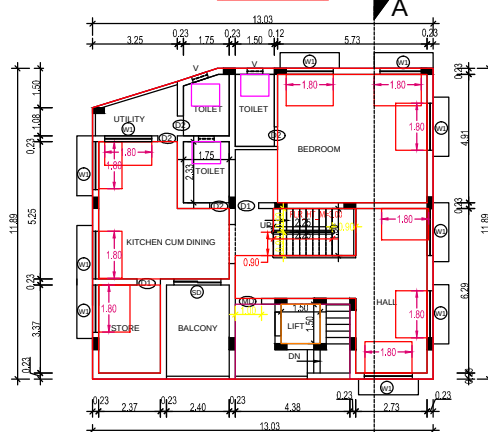
FIRST FLOOR PLAN (PROPOSED)
