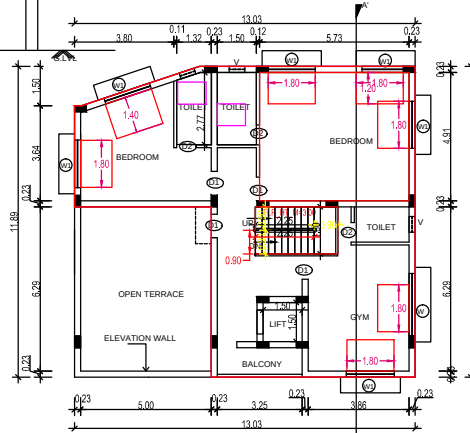
THIRD FLOOR PLAN (PROPOSED)
