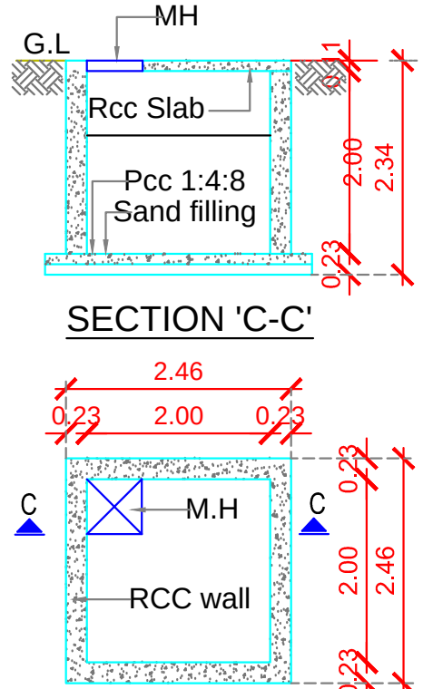
PLAN DRINKING WATER SUMP (Scientifically Closed)
