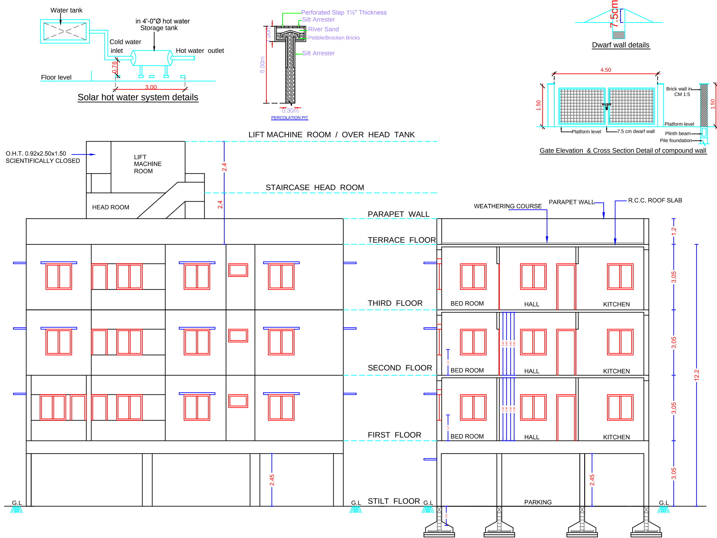
ELEVATION (PROPOSED)
