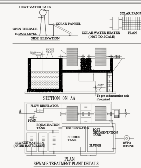
PLAN WASTE TREATMENT PLANT DETAILS
