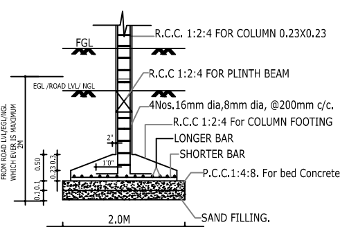
FOUNDATION DETAIL
