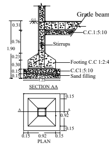
FOUNDATION DETAILS
