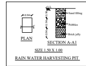
RAIN WATER HARVESTING PIT
