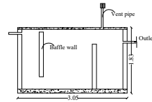
SEPTIC TANK DETAILS Size: 3.05 x 1.83 SCALE 1:100
