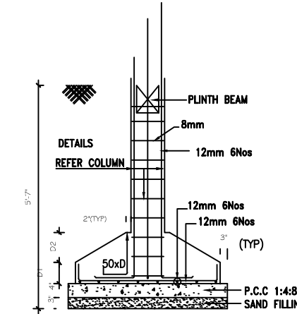
FOUNDATION DETAILS
