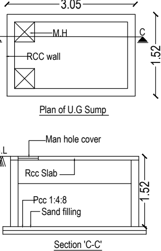
Section "C-C"
