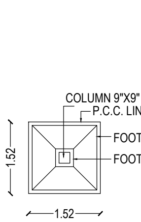
PLAN OF FOOTING
