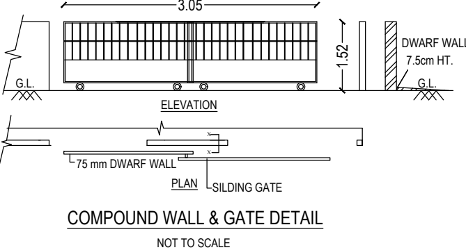
COMPOUND WALL & GATE DETAIL
