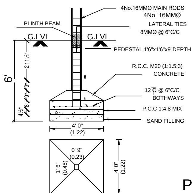
FOUNDATION DETAIL
