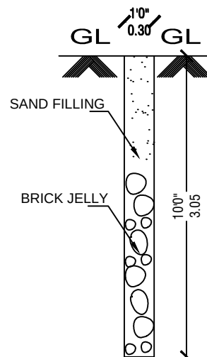
PERCOLATION PIT
