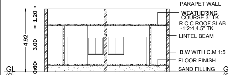
SECTION ON "SK"
