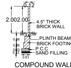
COMPOUND WALL
