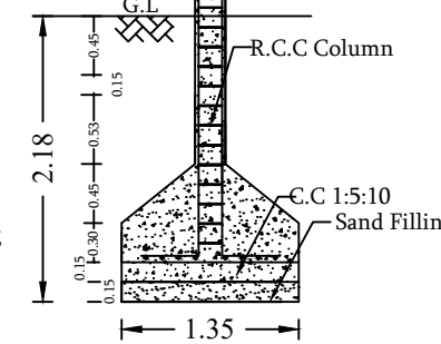
FOUNDATION DETAILS
