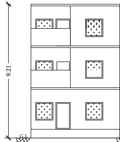
FRONT ELEVATION
