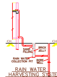
WELL AND RAIN WATER HARVEST SYSTEM
