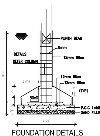
FOUNDATION DETAILS
