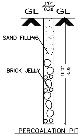
PERCOLATION PIT
