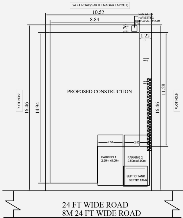
SITE PLAN
