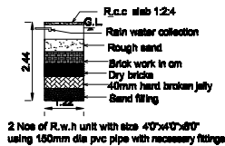
RAIN WATER HARVEST UNIT
