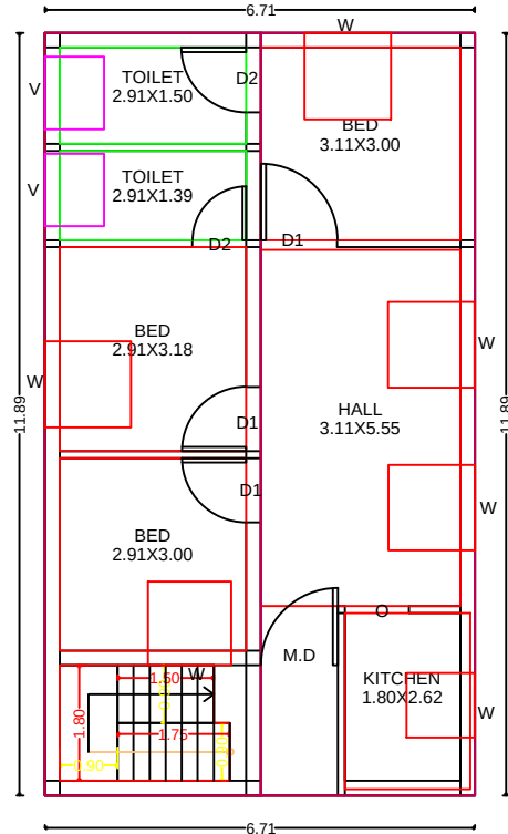
EXISTING & ADDITIONAL FIRST FLOOR PLAN
