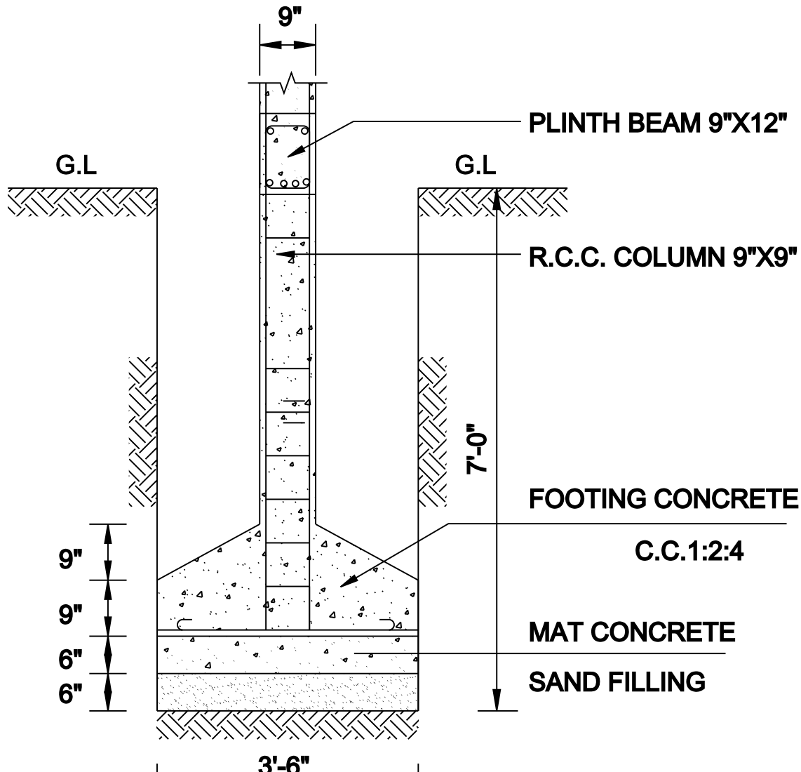
FOUNDATION DETAILS NOT TO SCALE
