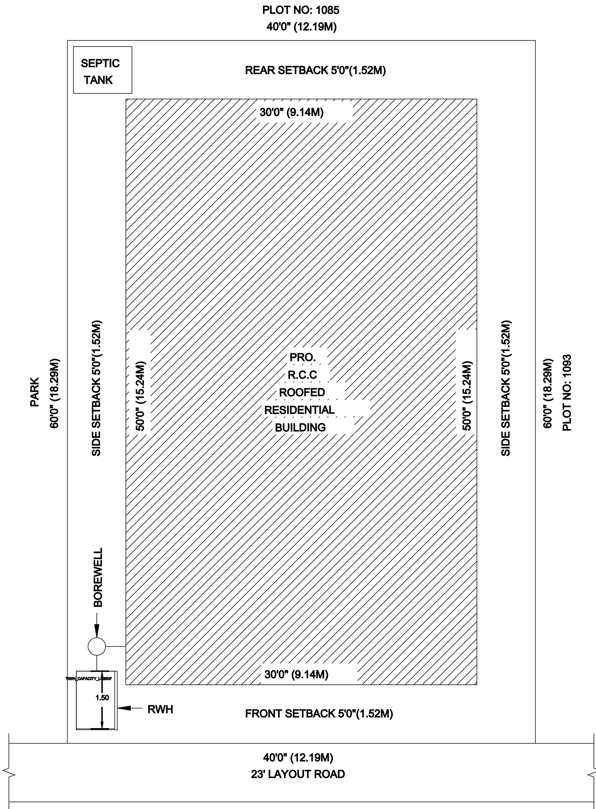
SITE PLAN
