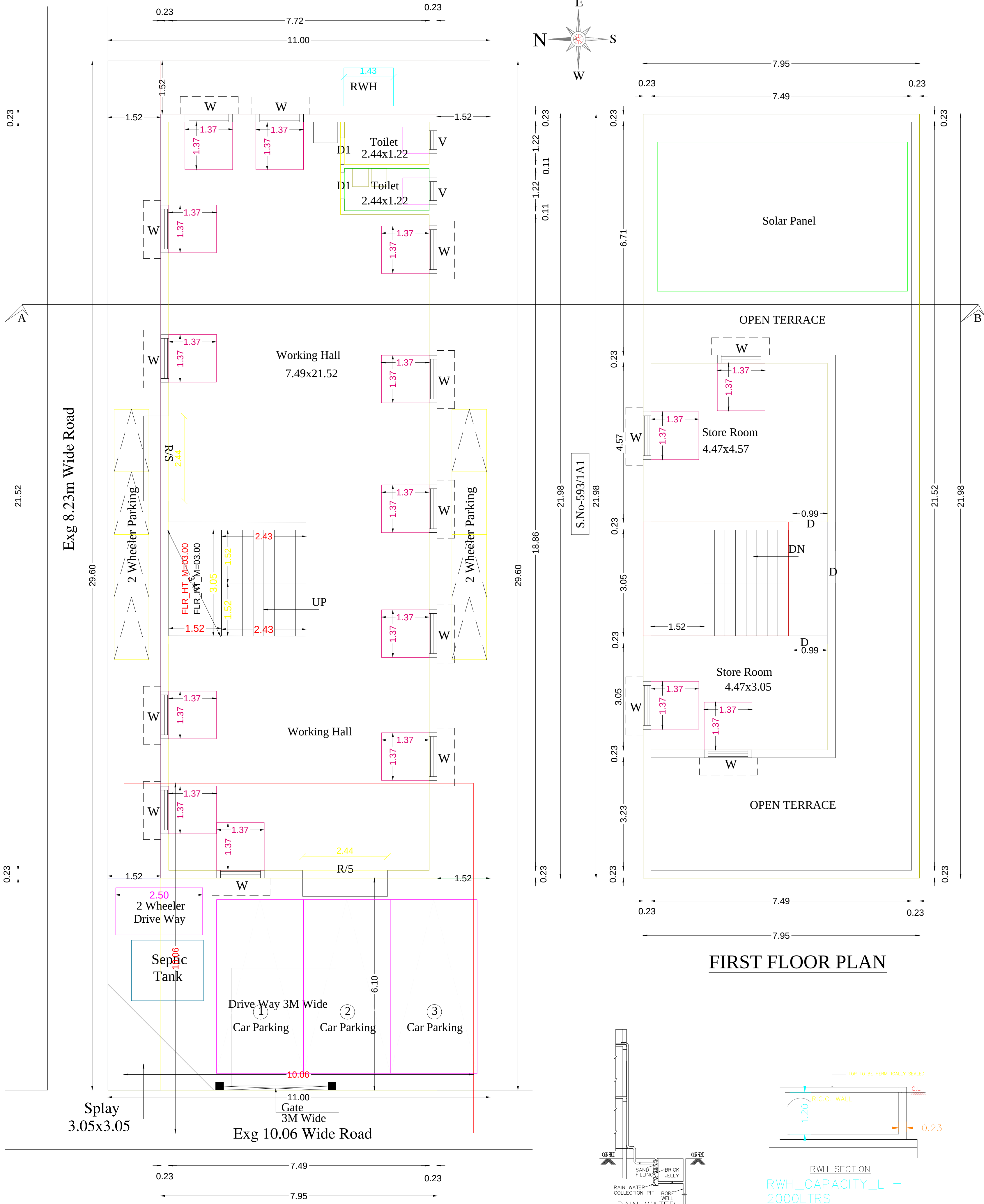
SITE CUM GROUND FLOOR PLAN
