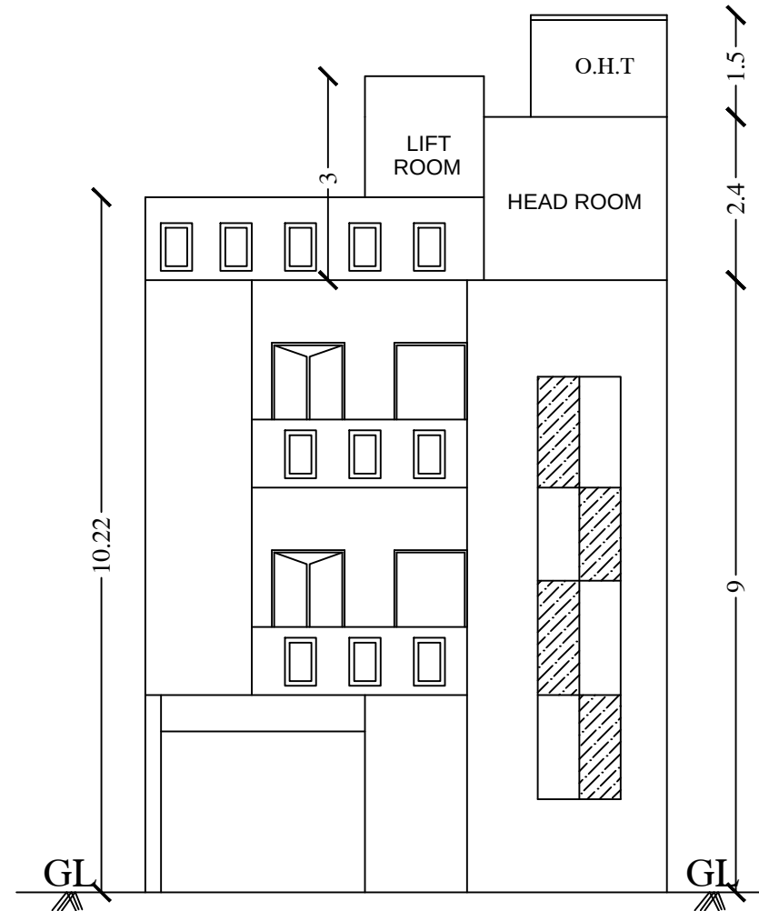
FRONT ELEVATION
