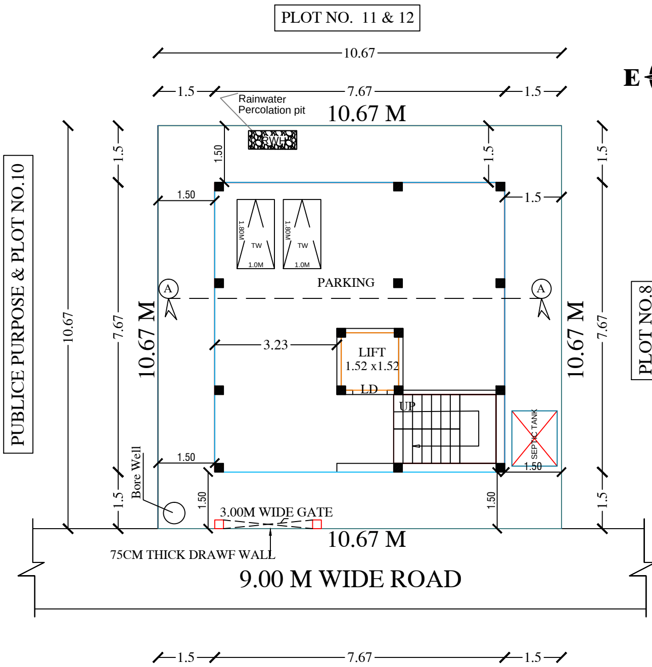
SITE CUM STILT FLOOR PLAN
