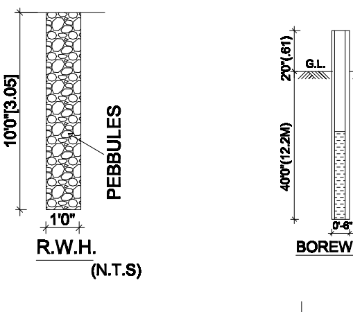
Pebbles Detail section
