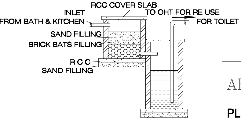
DETAILS THE RECYCLING OF WASTE WATER
