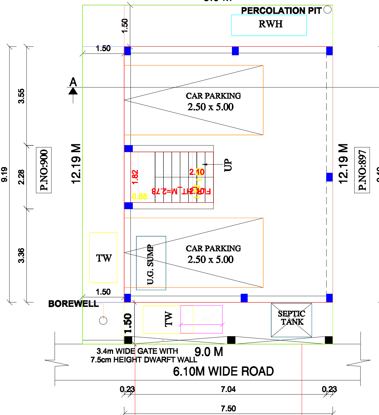
SITE CUM PRO.STILT FLOOR PLAN
