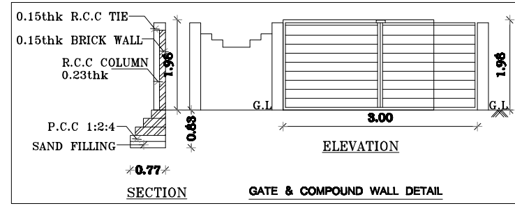
GATE & COMPOUND WALL DETAIL
