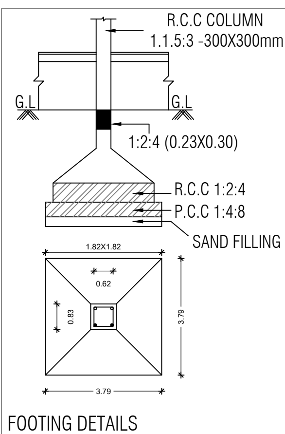
FOOTING DETAILS
