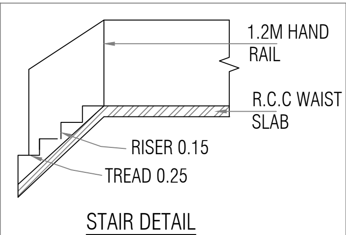
STAIR DETAIL
